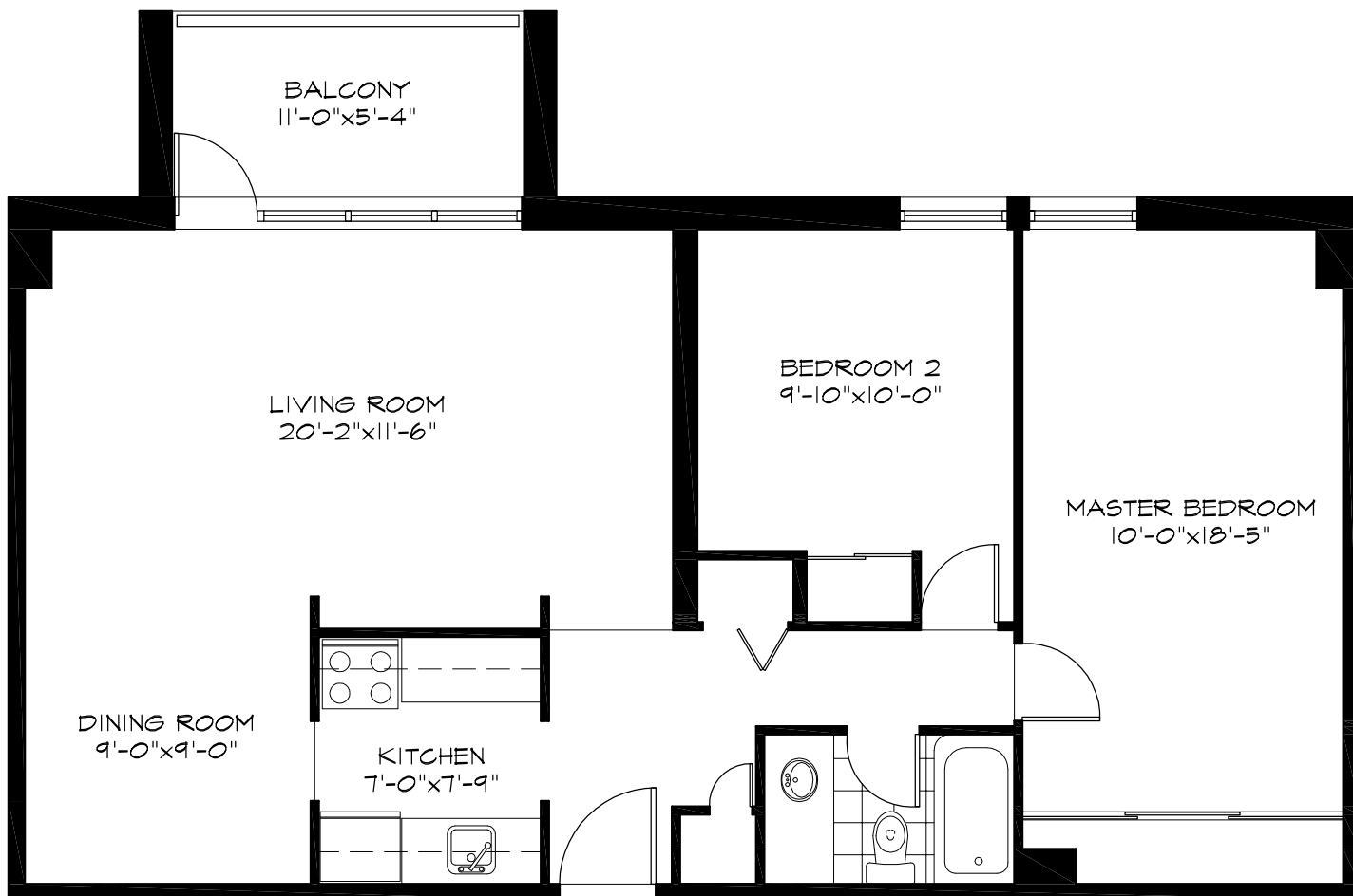
2 BEDROOM APARTMENT (TYPE 2) 100 VARLEY LANE
